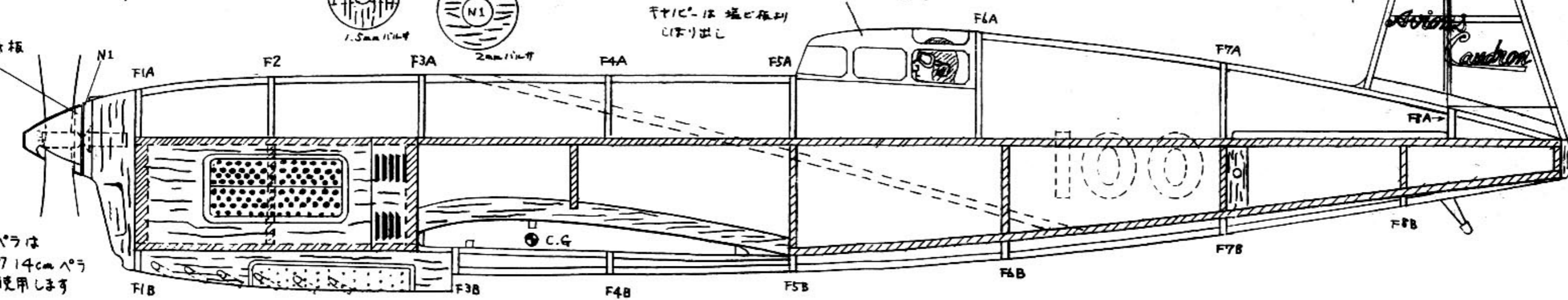
winner of THOMPSON, 1936 Peanut's Scale Caudron C. 460 Racer
